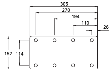
Baseplate S225, S225 Tall, S250, S250 Tall, S300
