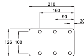
Baseplate S150, S175
