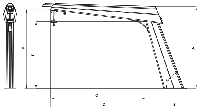
Baseplate S225, S225 Tall, S250, S250 Tall, S300
