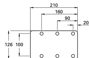
Baseplate S150, S175
